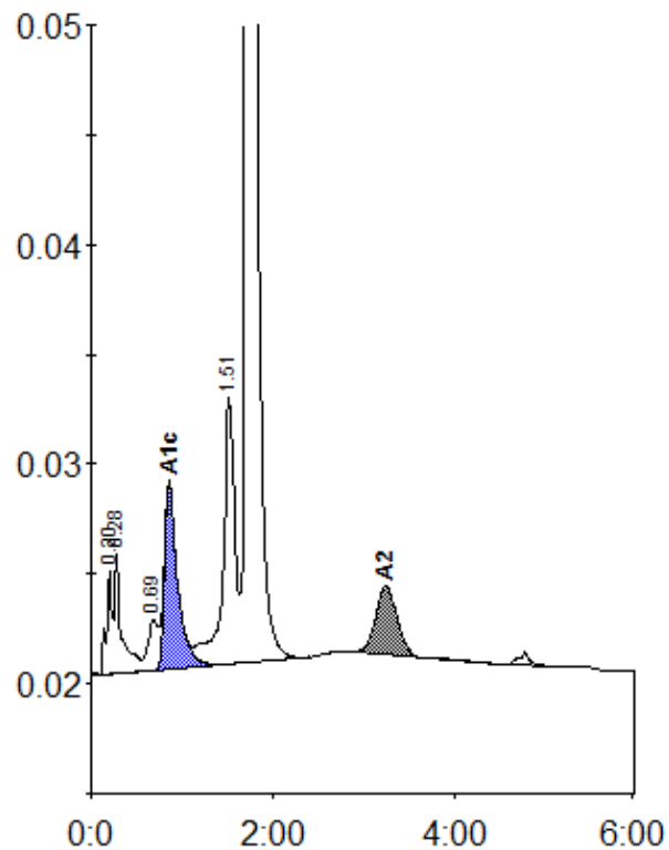
Peak table - ID: 2507021413
