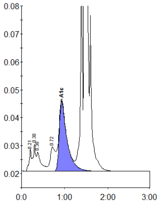
Peak table - ID: 10371012
