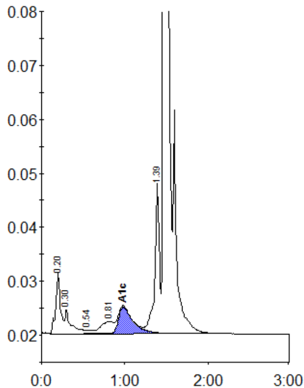
Peak table - ID: 10362080
