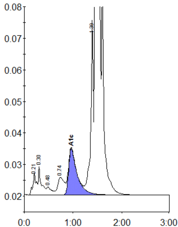
Peak table - ID: 10370307
