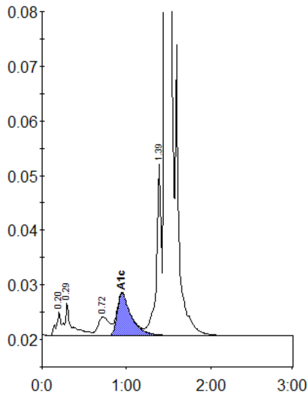
Peak table - ID: 10363349
