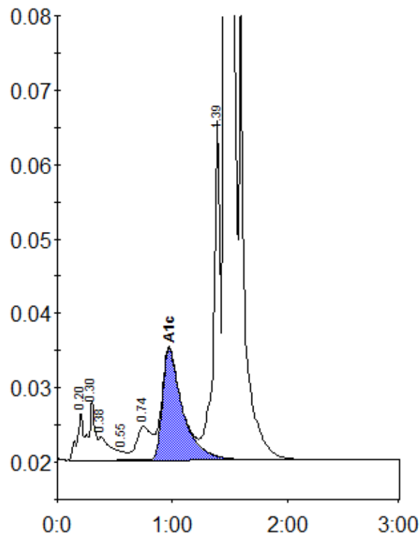
Peak table - ID: 10359840
