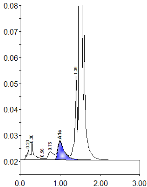
Peak table - ID: 10353698
