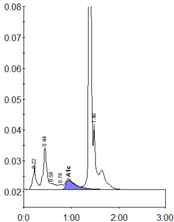
Peak table - ID: 10334897
