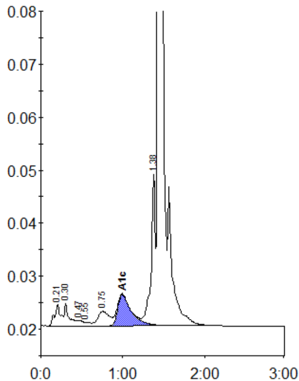
Peak table - ID: 10314495
