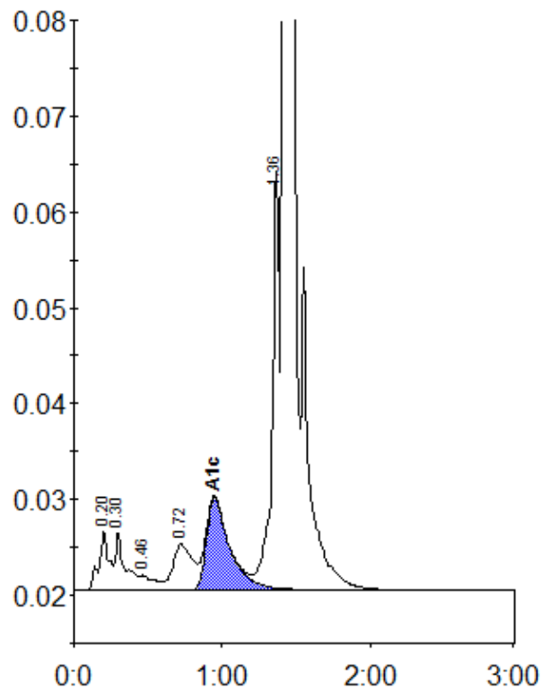
Peak table - ID: 10306661
