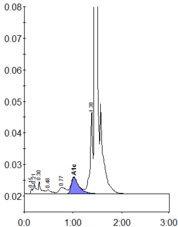
Peak table - ID: 10241813
