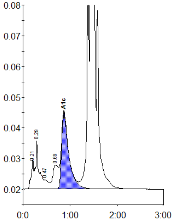
Peak table - ID: 10185052
