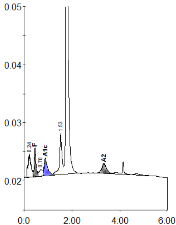
Peak table - ID: 10180298
