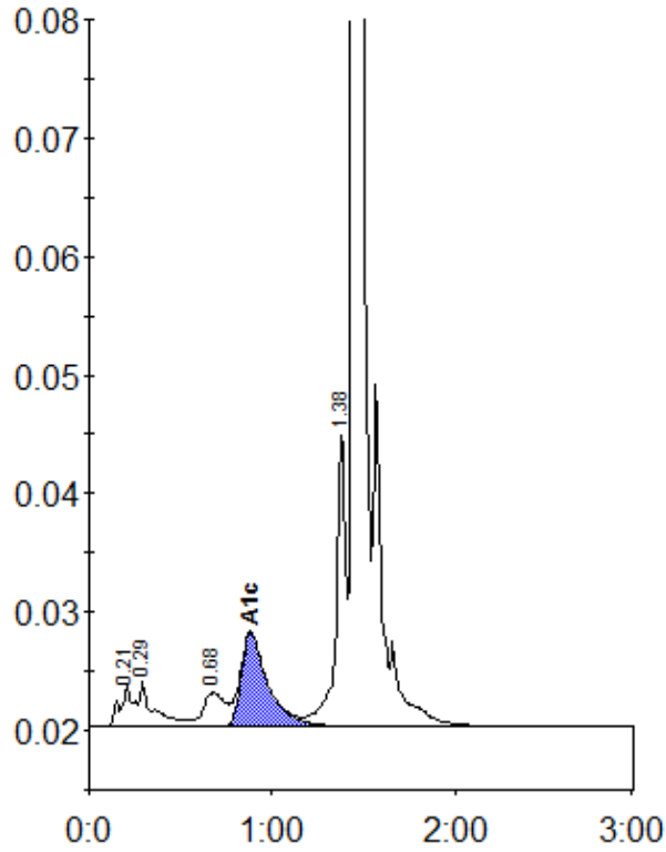
Peak table - ID: 10179557
