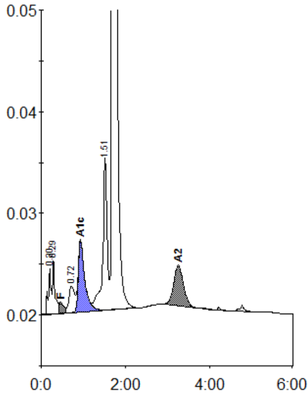
Peak table - ID: 10300577
