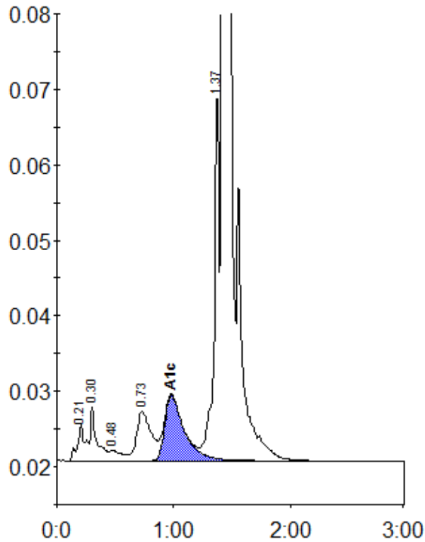
Peak table - ID: 10283835
