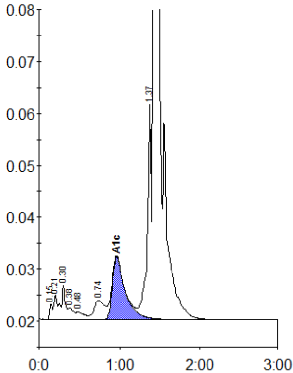
Peak table - ID: 10244422
