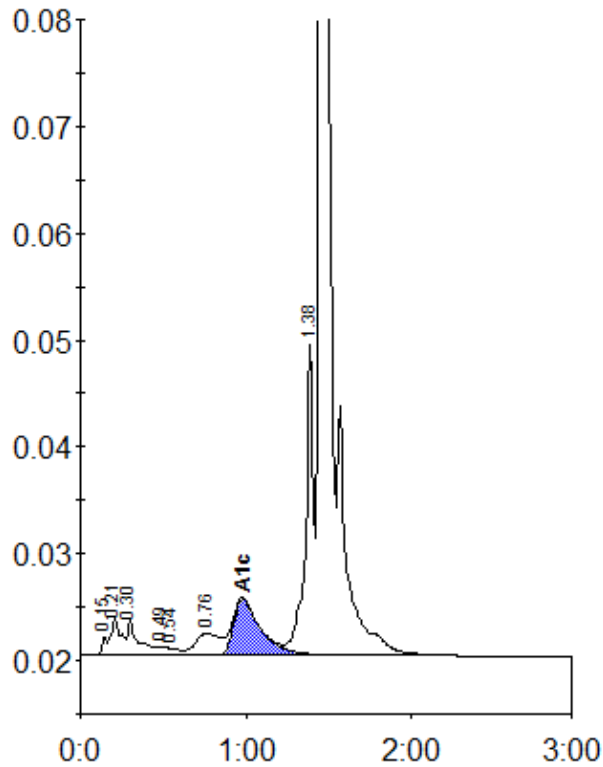
Peak table - ID: 10236124
