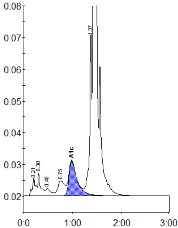
Peak table - ID: 10281724
