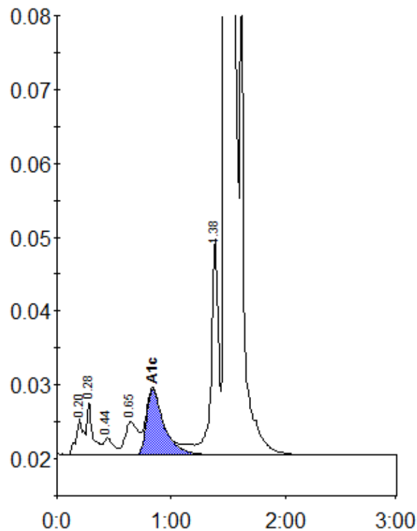
Peak table - ID: 10346669
