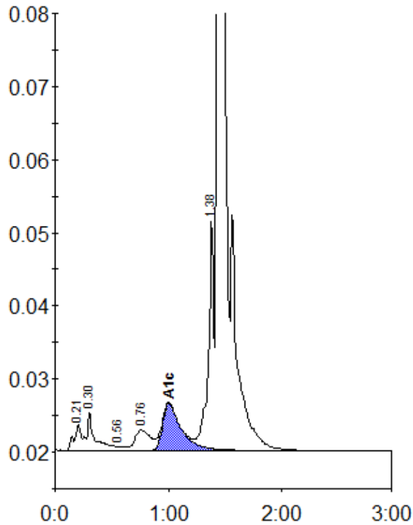
Peak table - ID: 10242951
