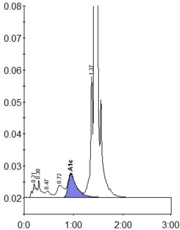
Peak table - ID: 10279940
