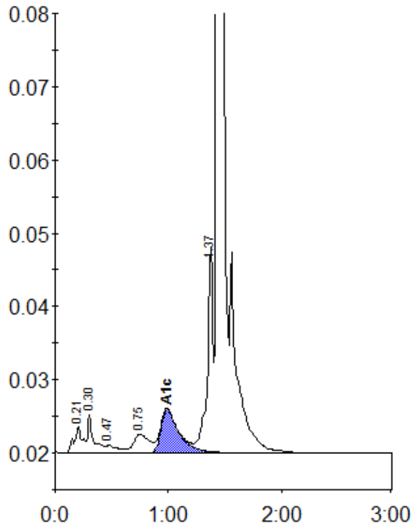
Peak table - ID: 10297162
