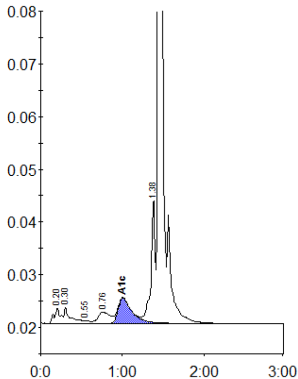
Peak table - ID: 10319986
