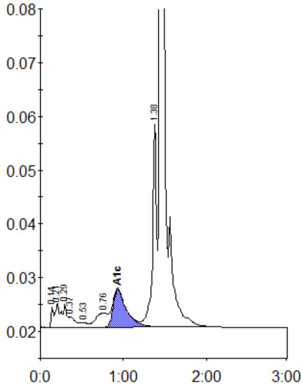
Peak table - ID: 10228507
