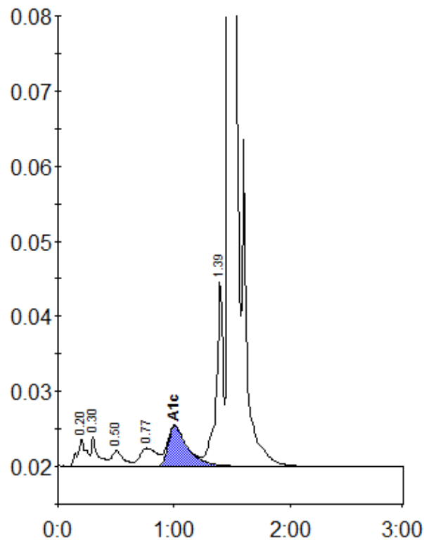
Peak table - ID: 10350314
