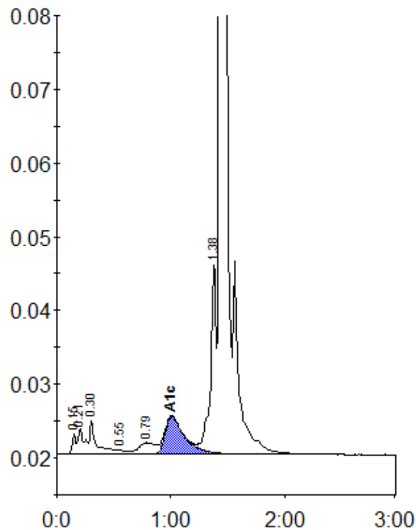
Peak table - ID: 10323349
