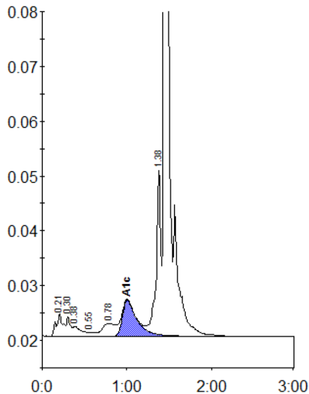
Peak table - ID: 10313218
