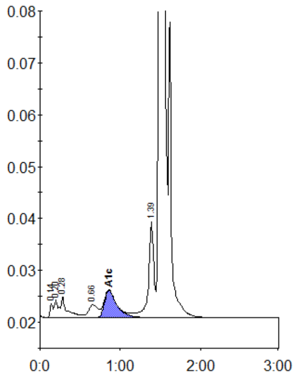
Peak table - ID: 10348249
