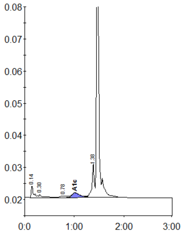
Peak table - ID: 10327816
