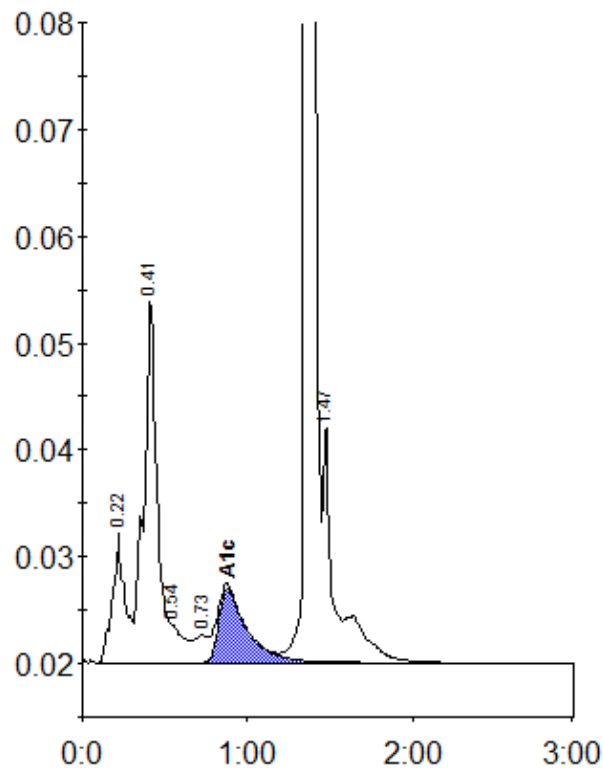
Peak table - ID: 10335838
