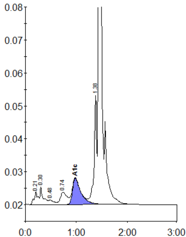
Peak table - ID: 10314938
