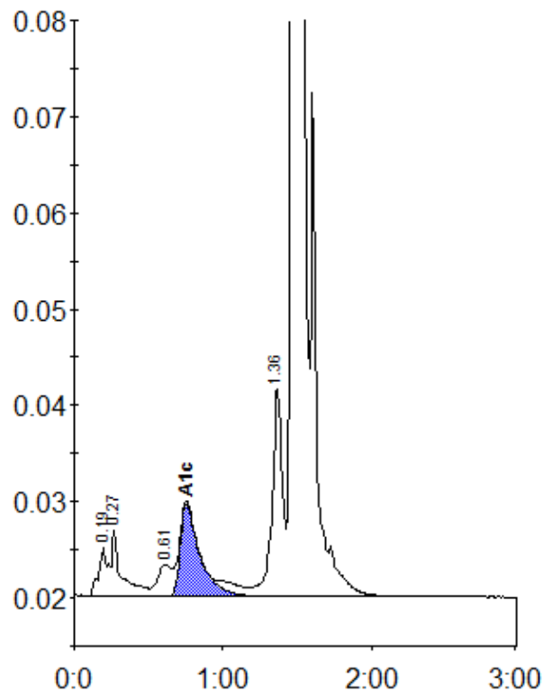
Peak table - ID: 10340946
