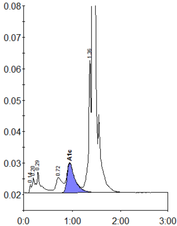
Peak table - ID: 10311260
