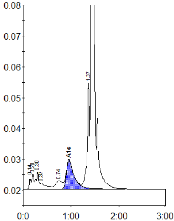
Peak table - ID: 10306786
