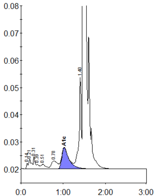
Peak table - ID: 10369706
