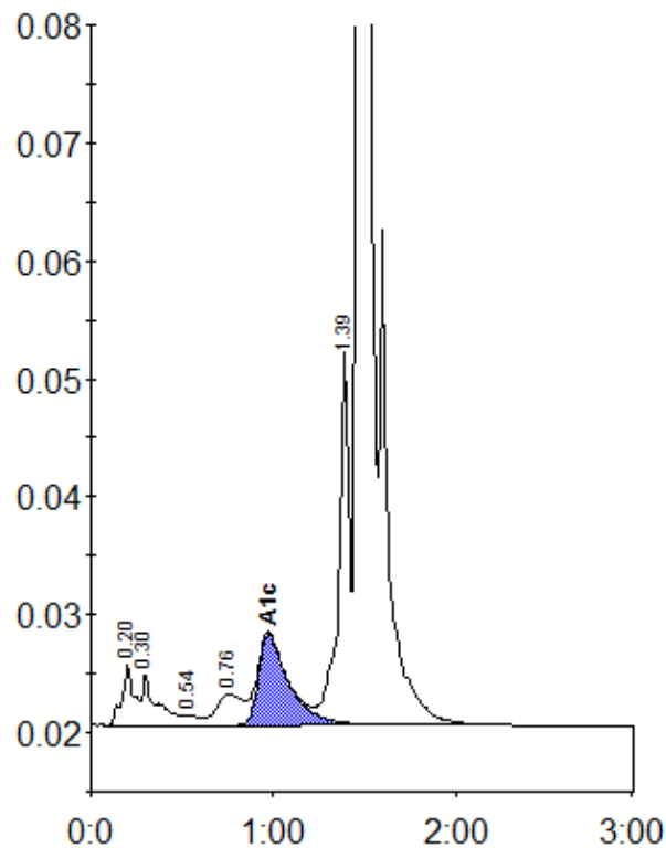
Peak table - ID: 10356718
