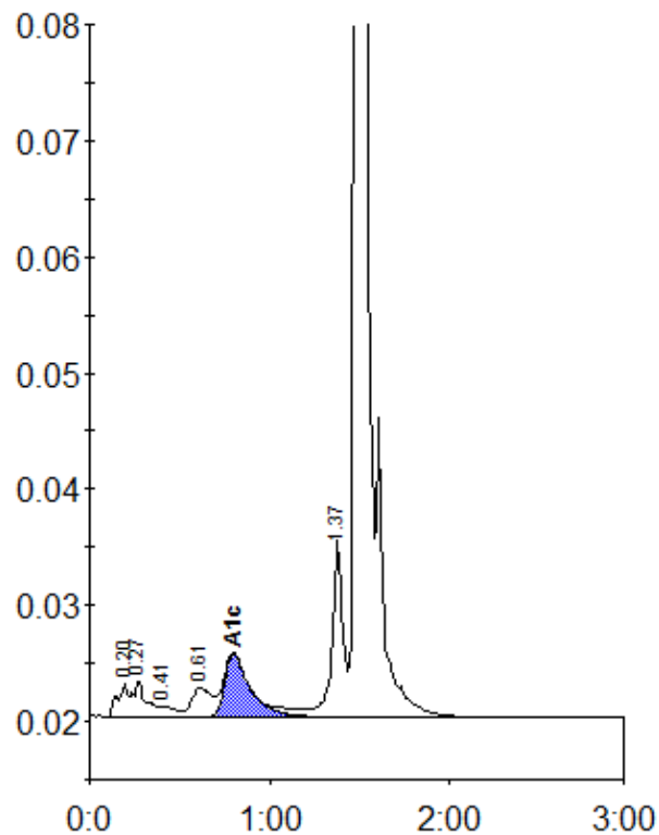
Peak table - ID: 10343108
