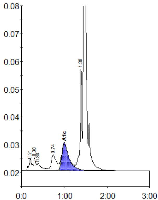
Peak table - ID: 10328958
