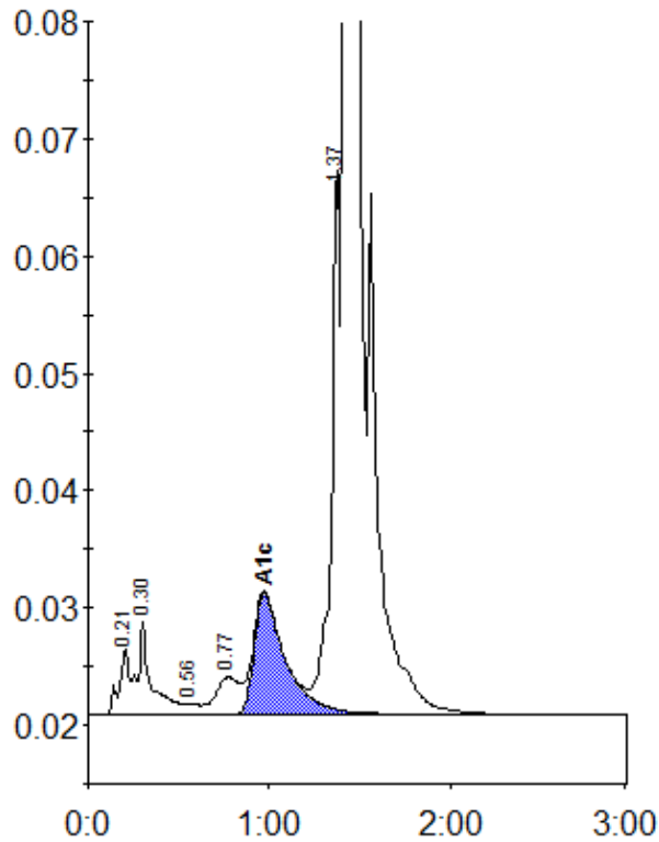
Peak table - ID: 10318577
