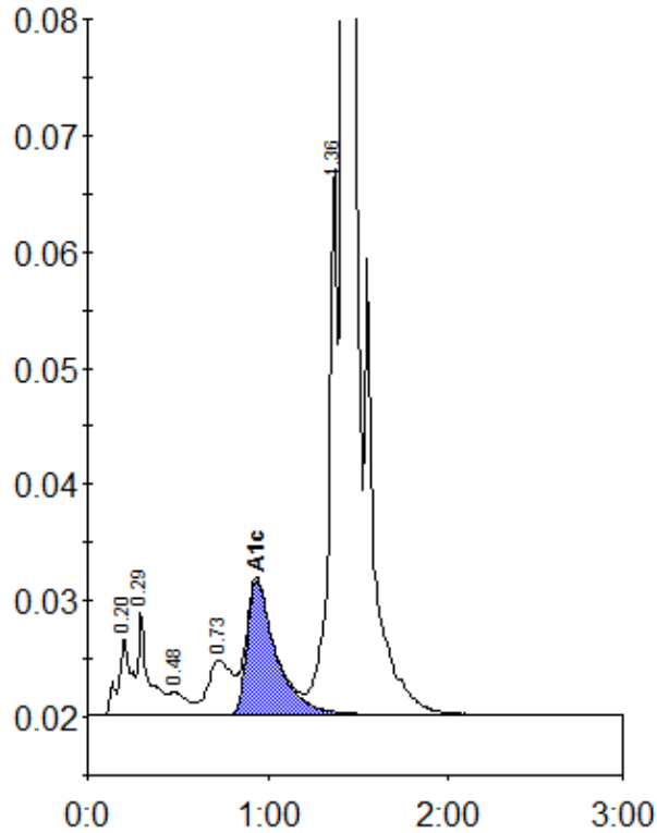
Peak table - ID: 10306924
