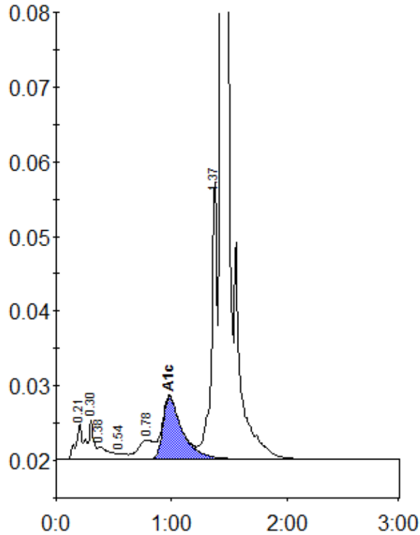
Peak table - ID: 10285217
