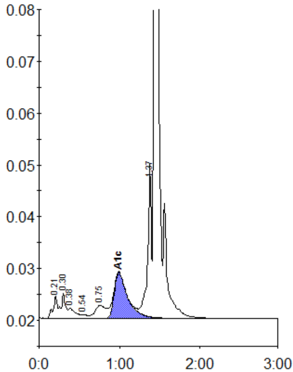
Peak table - ID: 10284607
