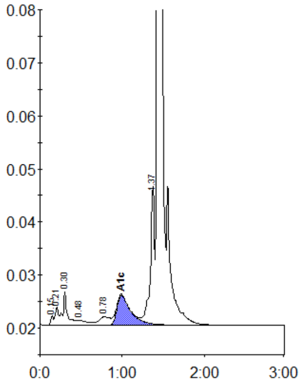
Peak table - ID: 10262710
