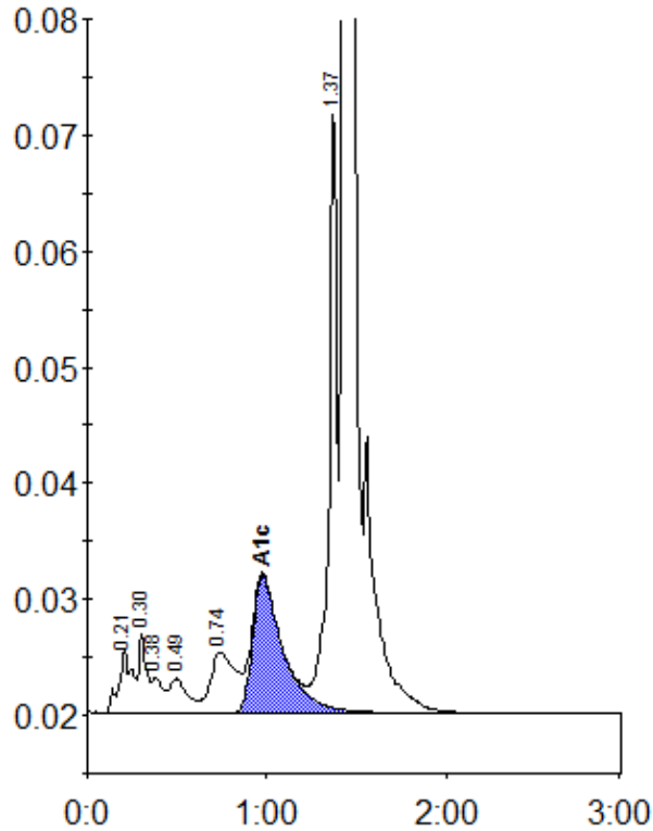
Peak table - ID: 10261751
