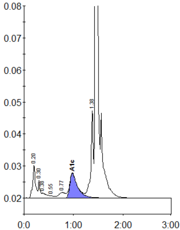
Peak table - ID: 10244831
