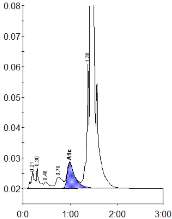
Peak table - ID: 10241935
