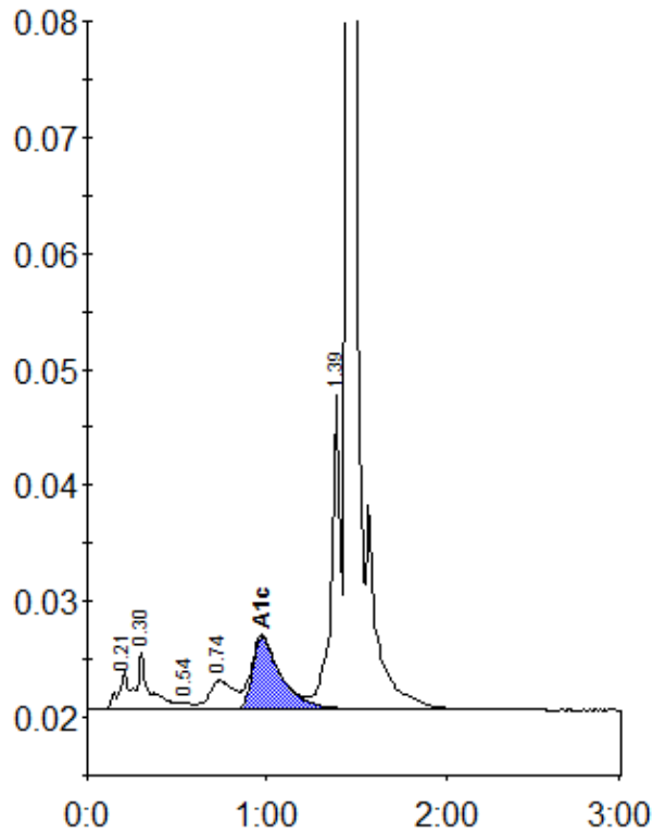
Peak table - ID: 10236980
