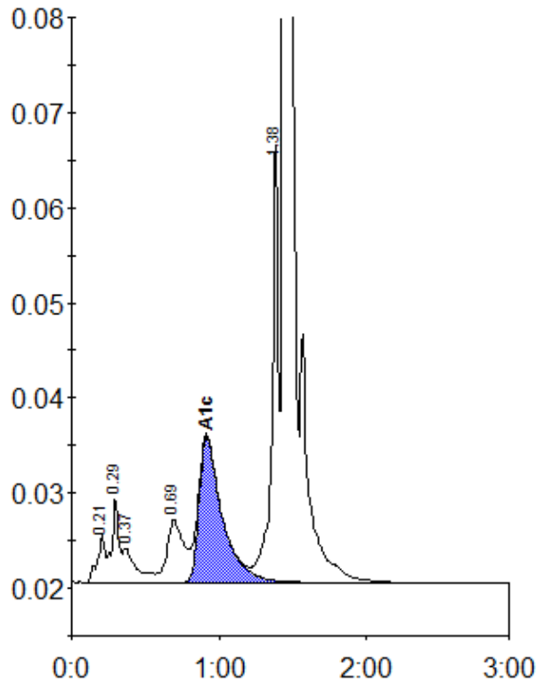
Peak table - ID: 10234873
