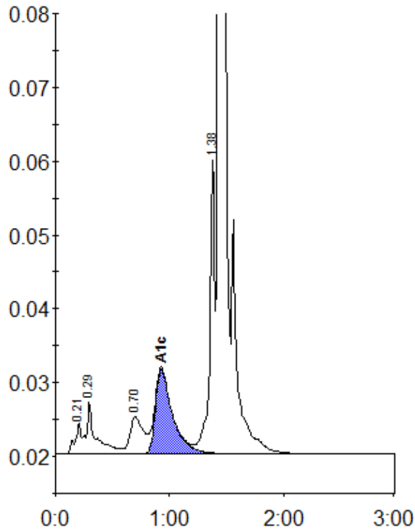
Peak table - ID: 10220502
